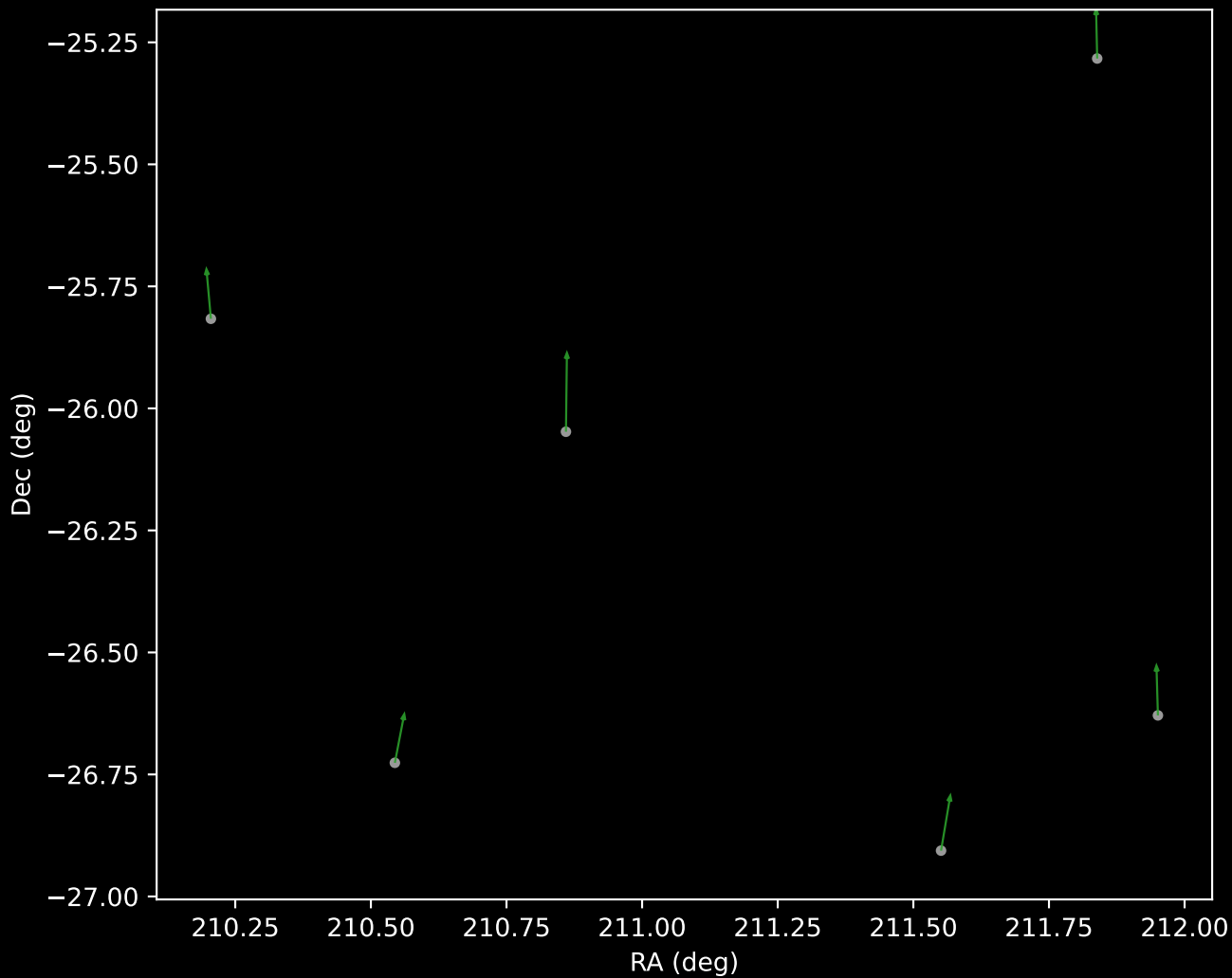
GALAH DR4 Cluster 4 Proper Motion Vectors (n=6)
