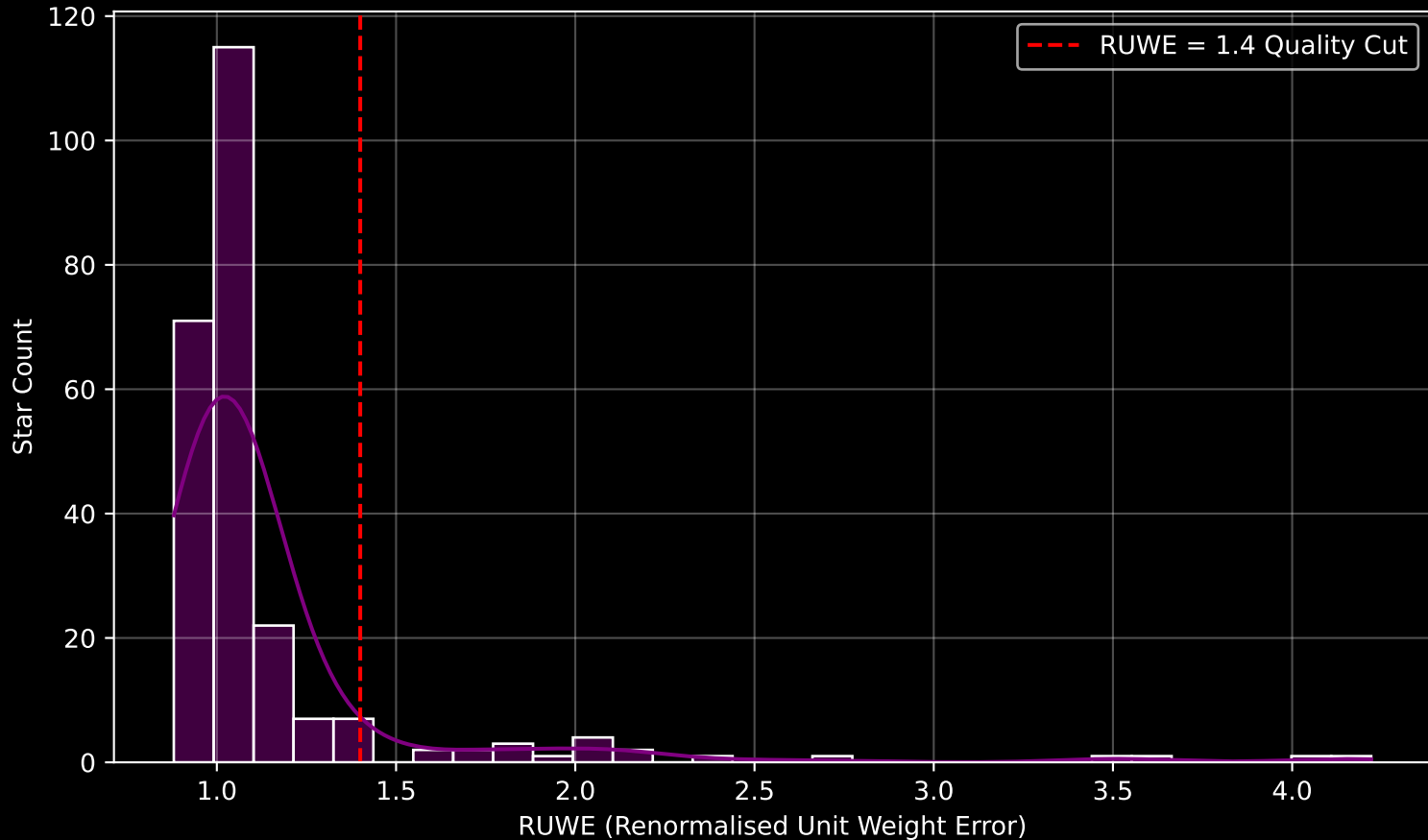
GALAH DR4 Field [8390] RUWE Distribution (n= 242)
