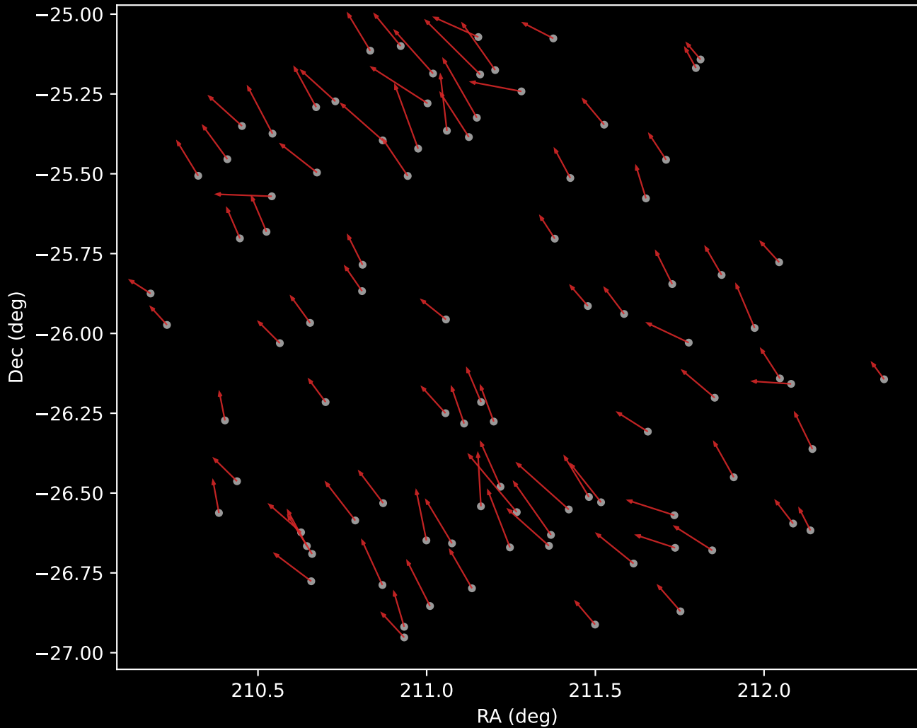
GALAH DR4 Cluster 6 Proper Motion Vectors (n=91)
