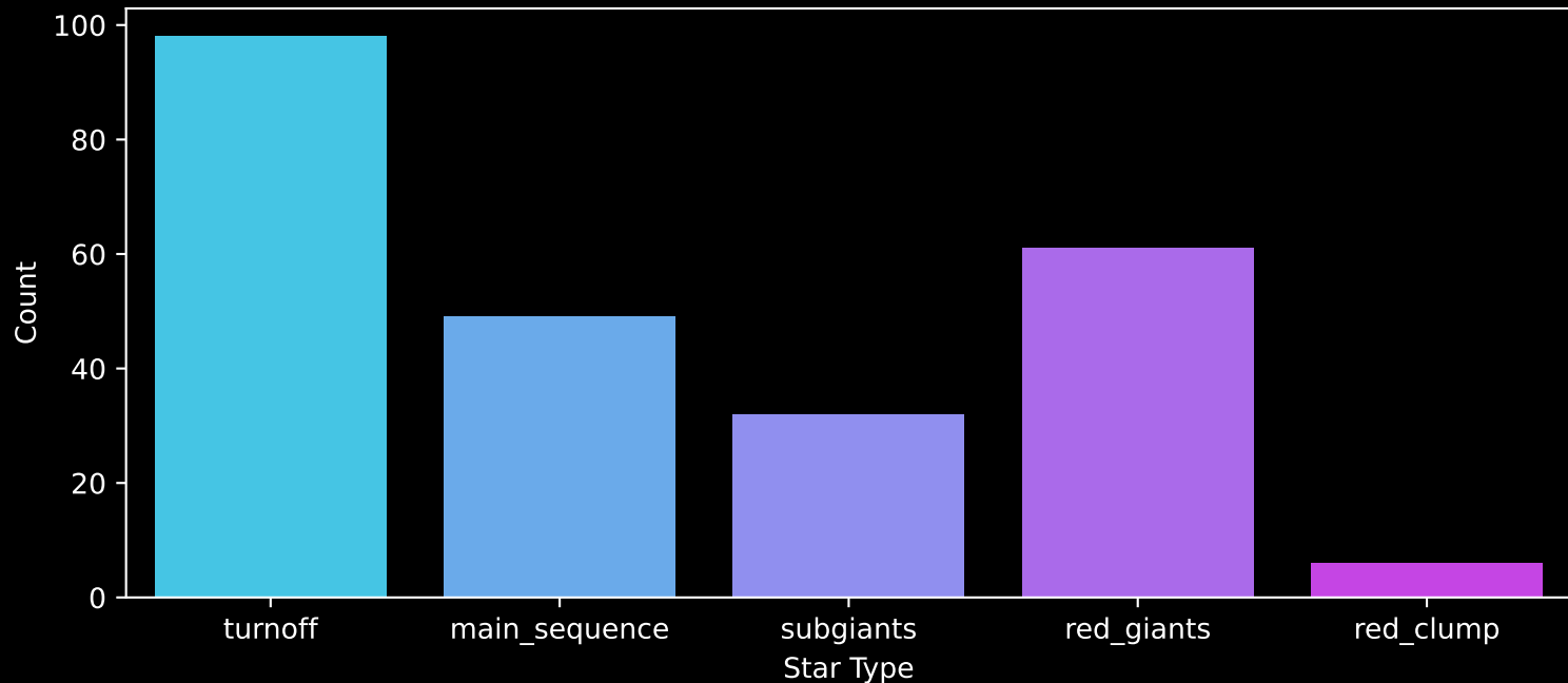
GALAH DR4 Field: [8390] Count plot of Star Type
